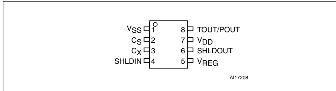
Figure 3. UFDFPN8 pinout
